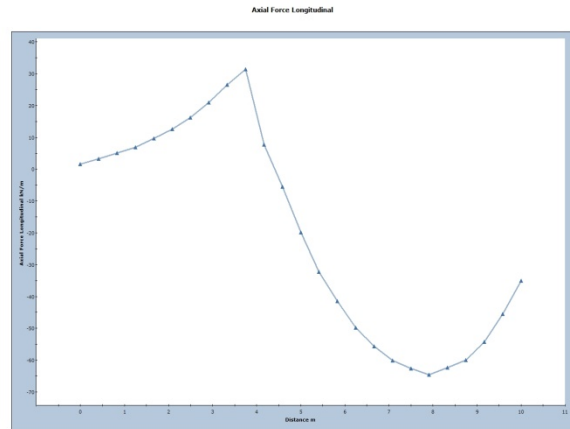
Figure 1-8: Model B axial force along liner in RS 2 (left) and RS 3
