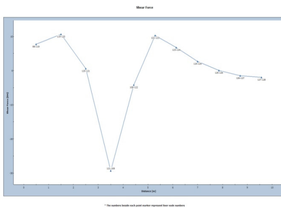
Figure 1-10: Model B shear force along liner in RS 2 (left) and RS 3
