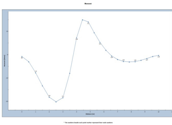
Figure 1-9: Model B moment along liner in RS 2 (left) and RS 3
