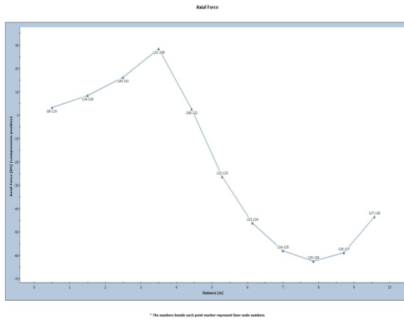
Figure 1-8: Model B axial force along liner in RS 2 (left) and RS 3
