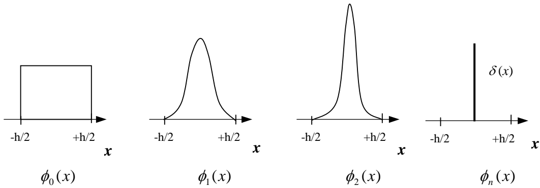
Figure 4.2: Interpolation functions
