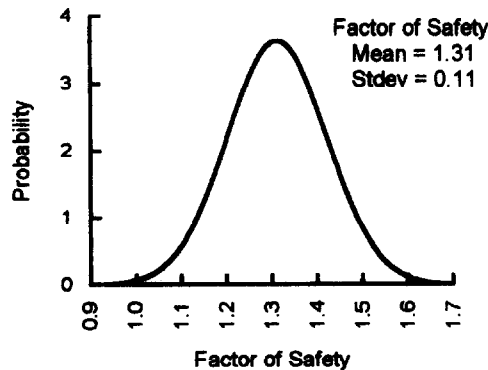
Fig. 4. Normal distribution for factor of safety of slope defined in Fig. 3.
