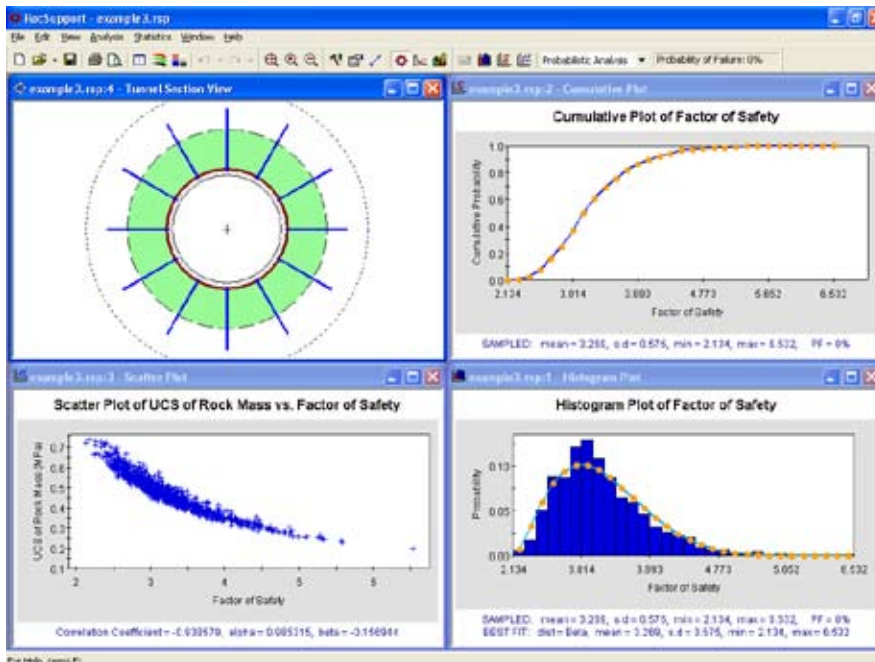
Display of probabilistic analysis results – histogram, cumulative and scatter plots. Tunnel section view also shown.
