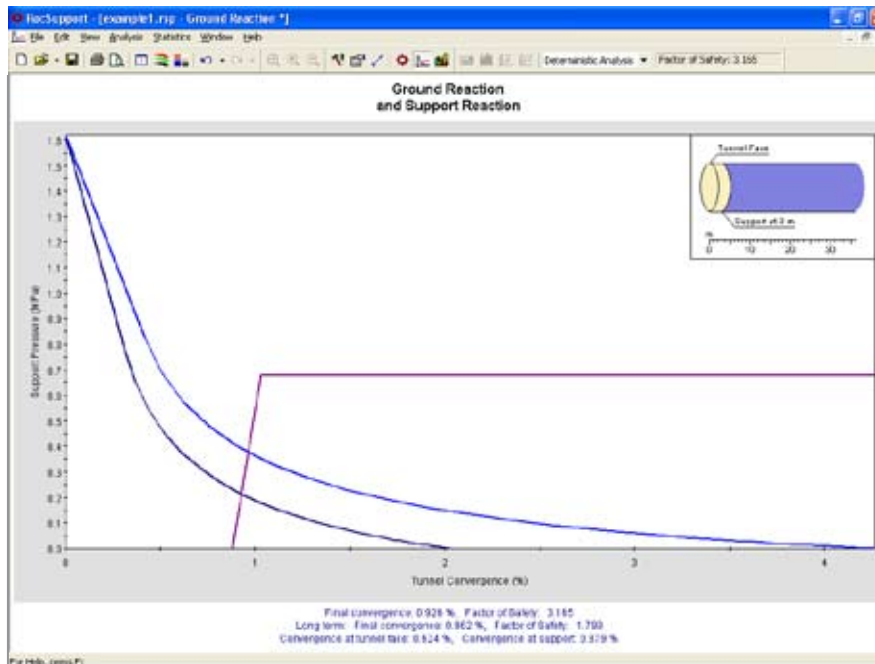
Ground reaction curves (short term and long term) and support reaction. The intersection of these curves determines the safety factor of the support.
