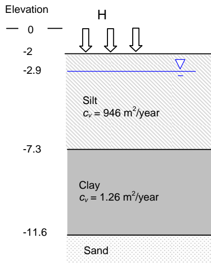
Figure 2. Two-layer model from Lambe and Whitman (1979, Example 27.2).
