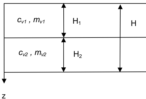
Figure 7. Geometry of two layer consolidation problems.
