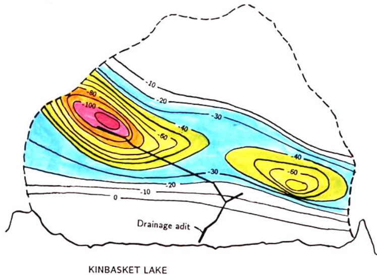
Figure 2. Contours of water level reduction (m) as a result of the implementation of drainage in Dutchman's Ridge.
