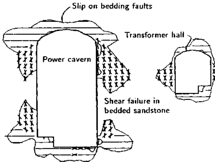
Figure 5. Predicted zones of over-stress along faults and in bedded sandstone surrounding the power cavern and transformer hall of the Mingtan Project.
