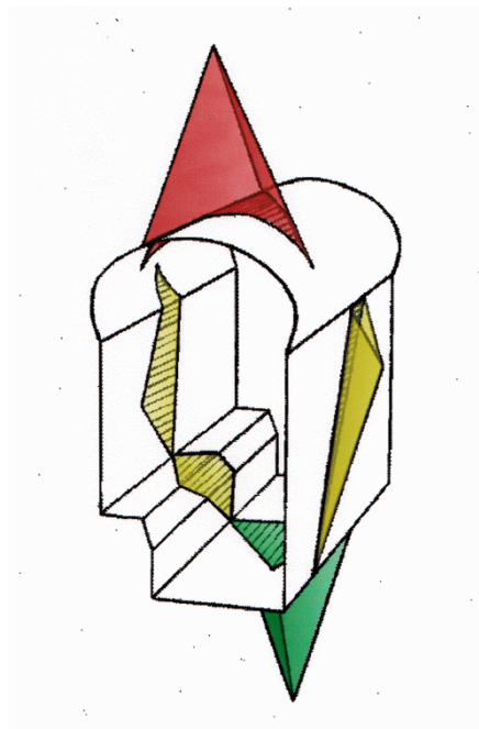
Figure 4. Perspective view of Rio Grande power cavern showing potentially unstable wedges in the roof, sidewalk, bench and floor.
