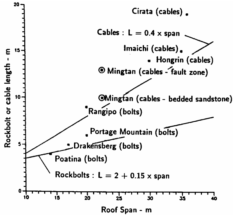
Figure 6. Lengths of rockbolts and cables used for roof support in some large caverns in weak rock. Equations defining trend lines were suggested by Barton (1989).
