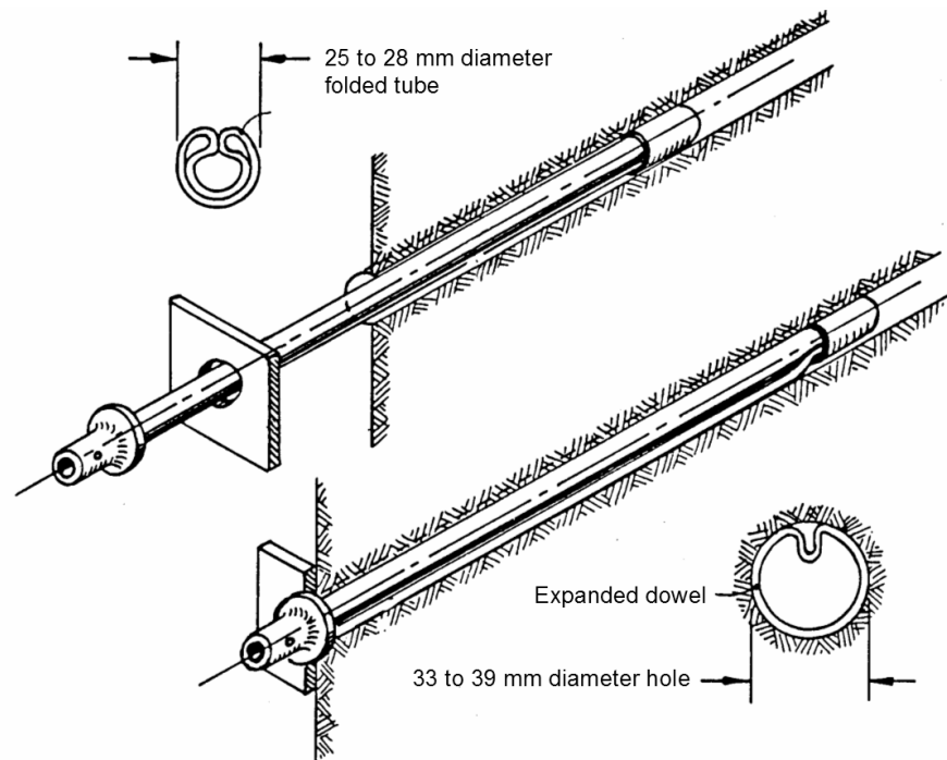
Figure 8: Atlas Copco 'Swellex' dowel.
