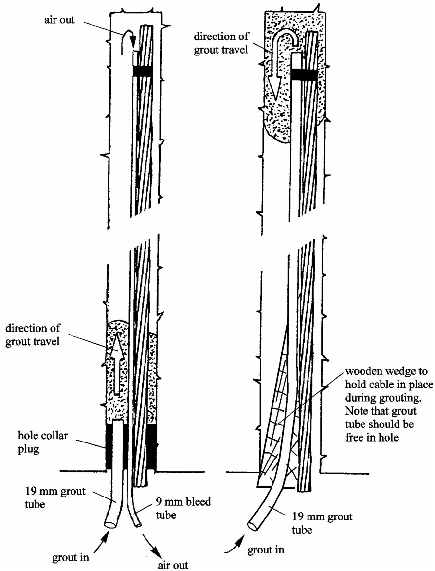
Figure 14: Alternative methods for grouting cables in upholes.
