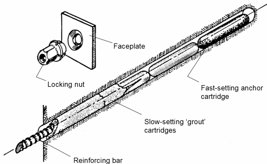
Figure 4: Typical set-up for creating a resin anchored and grouted rockbolt. Resin grouting involves placing slow-setting resin cartridges behind the fast-setting anchor cartridges and spinning the bolt rod through them all to mix the resin and catalyst. The bolt is tensioned after the fast-setting anchor resin has set and the slow-setting resin sets later to grout the rod in place.
